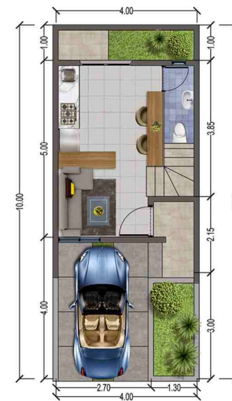
LANTAI 1
